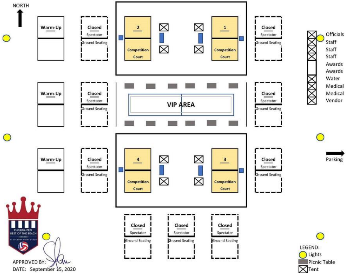
Hickory Point Beach Sand Volleyball Complex - Site Plan 21 Total Courts - 4 Court Pro Event Layout v2
